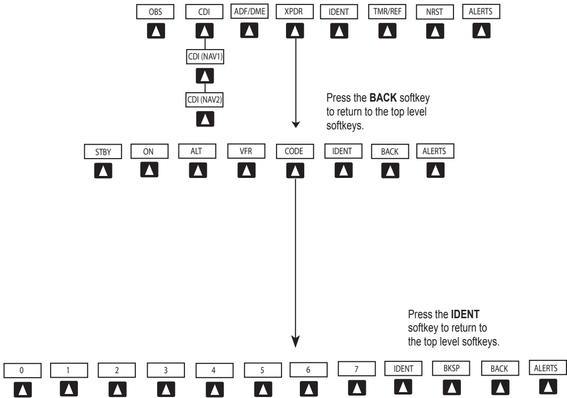
Figure 3.3.5 PFD Softkey Flow Chart – 3
