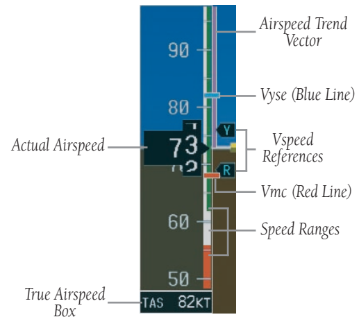
Figure 3.4.1 Airspeed Indicator
