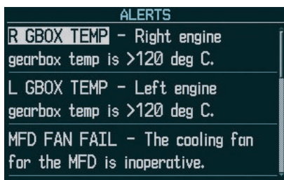
Figure 3.8.1 Alerts Window
