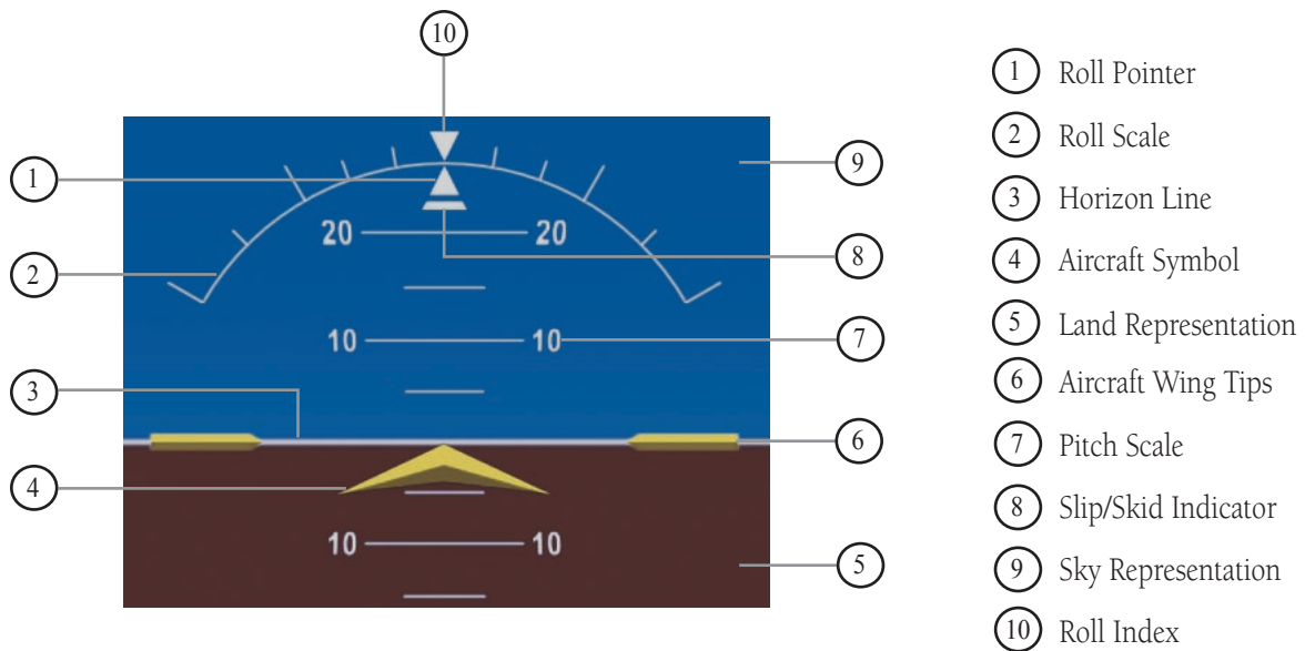
Figure 3.4.3 Attitude Indicator
